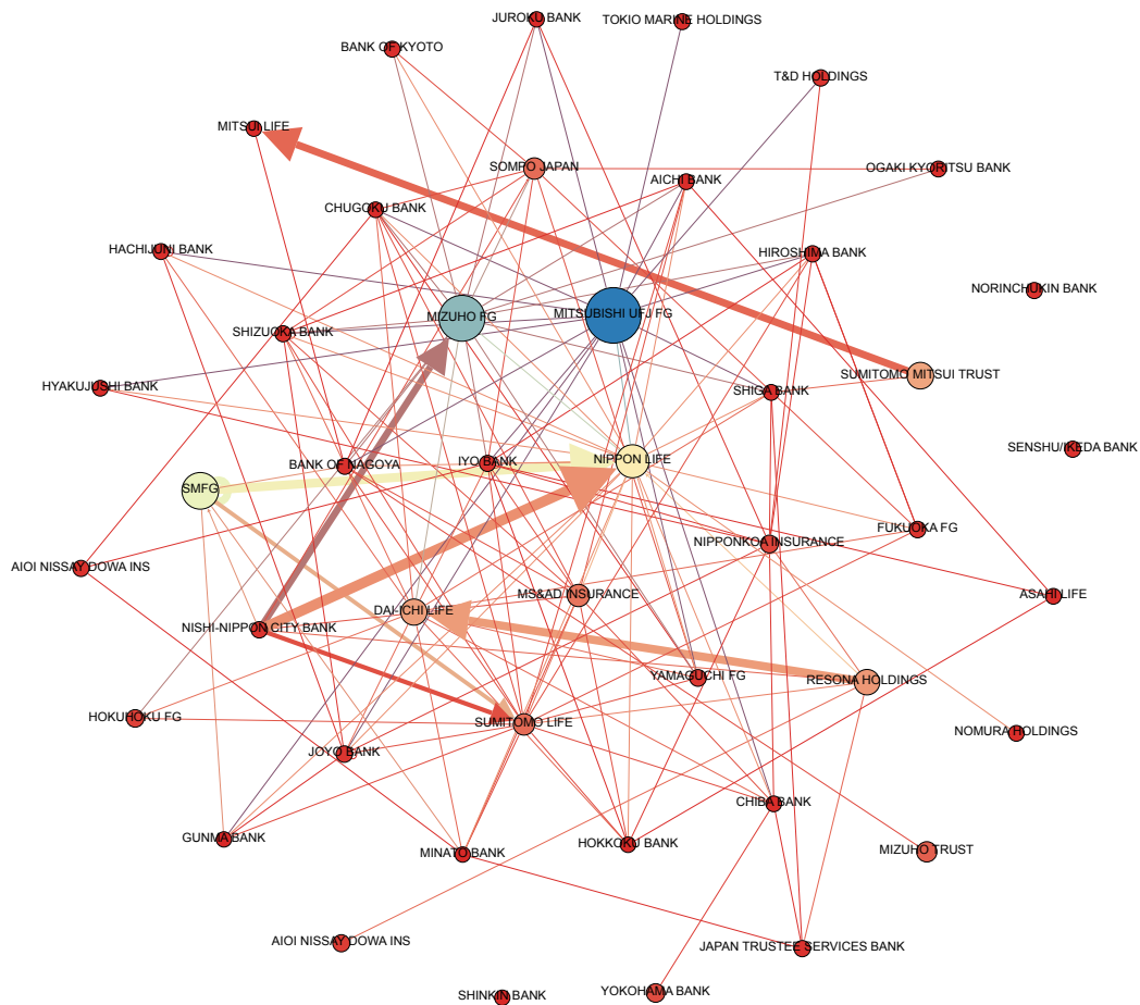
Figure 6: Directed graph of degrees over 70, end of March 2009 (just after the bankruptcy of Lehman Brothers)
